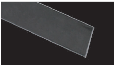
C.12003BL - Aluminio- Aluminium (25x3mm) (202 g/m) C.12000 - F.Vidrio-Fiberglass-Verre (25x4mm) (180 g/m)
