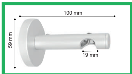
Soporte Pared 19mm
