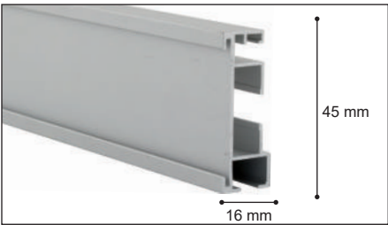
Perfil Inter Inter Profile / Inter Rail
