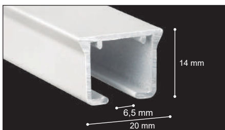
Riel Track / Rail
