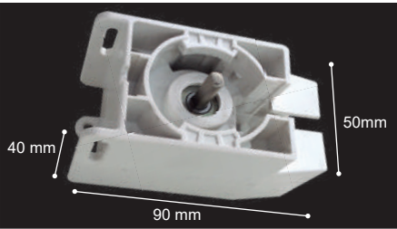
Cantonera Motor RM09-1000
